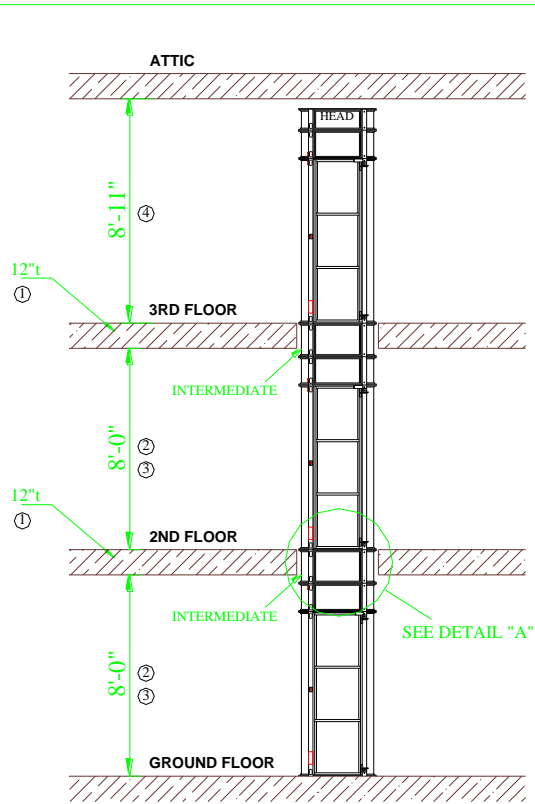
VIEW "A-A"
